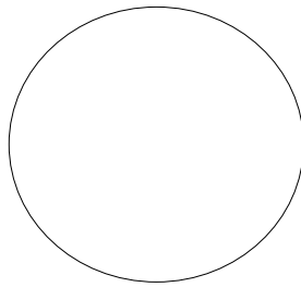
Figure 1 - working toward Venn Diagram for "All dogs are mammals"
