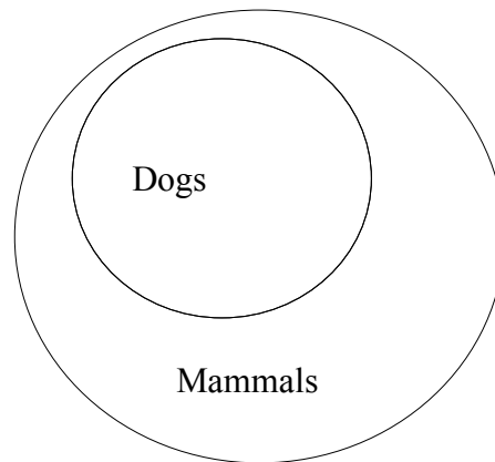
Figure 3 - the way Math/CS would draw this! (All Dogs are Mammals)
