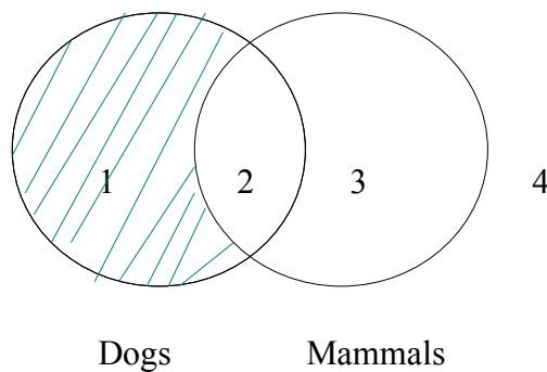
Figure 4 - the way a Logician would draw this! (All Dogs are Mammals)
