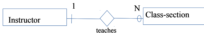
Figure 7 - ERD showing relationship class teaches' minimum cardinality between the entity classes of Instructor and Class-section
