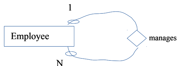
Figure 1 - ERD showing recursive relationship Employee-manages-Employee
