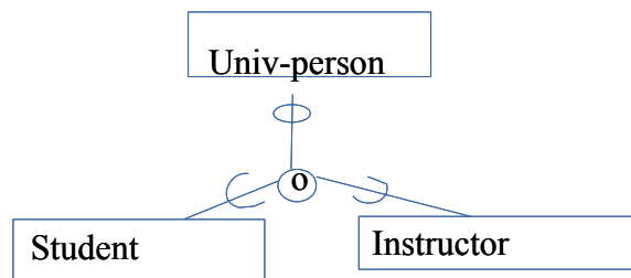
Figure 5 - ERD showing supertype entity class Univ-person with two subtype entity classes Student and Instructor
