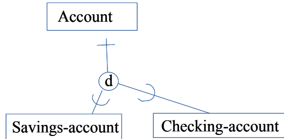
Figure 4 - ERD showing supertype entity class Account with two subtype entity classes Savings-account and Checking-account
