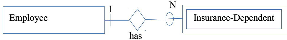
Figure 3 - ERD showing 1:N relationship Employee-has-Insurance-Dependent, including showing Insurance-Dependent as a weak entity class
